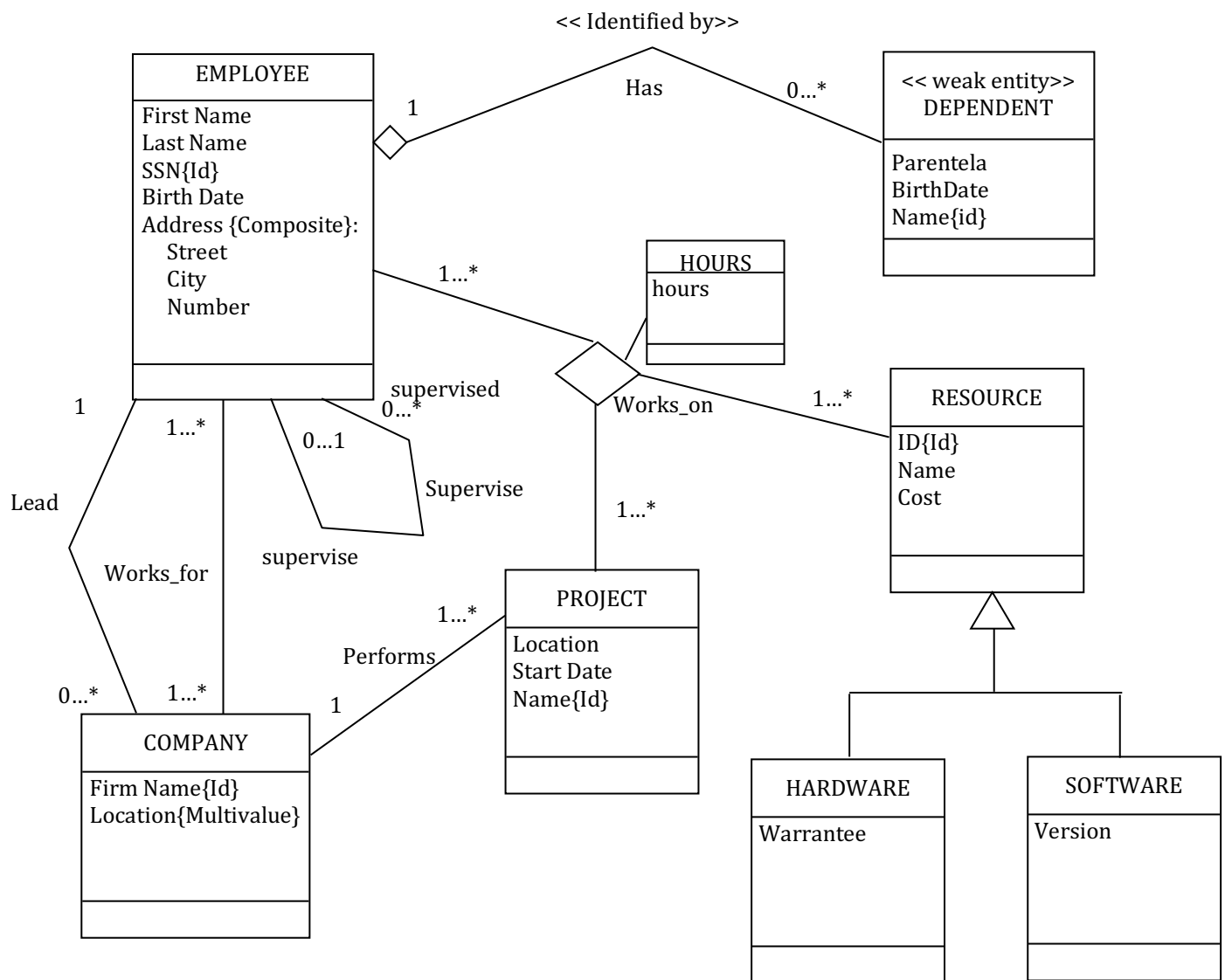
Figure 1: The UML class diagram of a system managing company information
